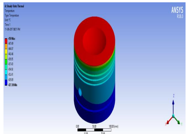
Figure 8 shows total heat flux piston with Crown as BRONZE.
