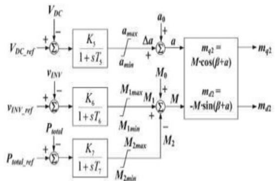
Fig-7: control block diagram of the modulation indices of grid VSI
