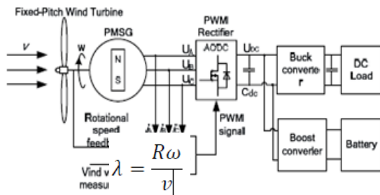
Fig-2: Topology of non grid connected wind energy conversion system
