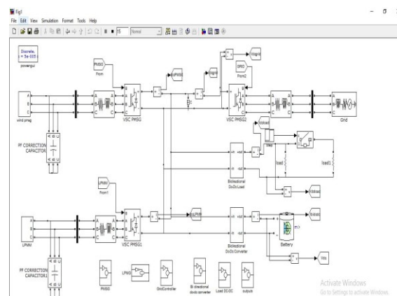
Fig 8. MATLAB/SIMULATION diagram of proposed wind and wave system
