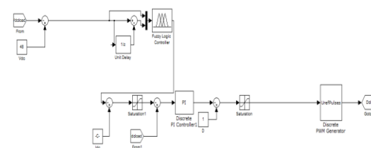
Fig 8. MATLAB/SIMULATION diagram of proposed wind and wave system
