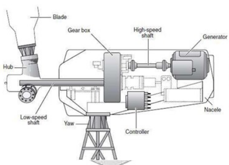
Fig-3: Horizontal axis wind mill
