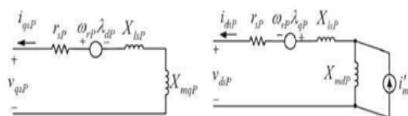
Fig-4: q-d axis equivalent circuit model of the studied wind PMSG
