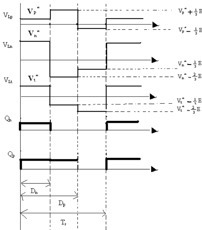
Fig.4 Inductor voltage waveforms for the converter during condition d_p > d_n
