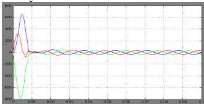
Fig.10 Source current with fuzzy one cycle control
