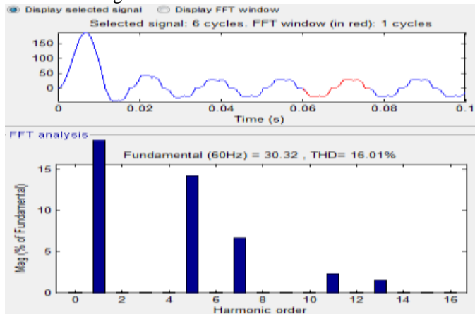
Fig.9 Total Harmonic Distortion without shunt filter
