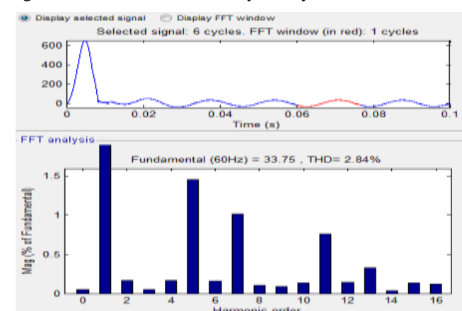
Fig.11 THD with fuzzy one cycle controller
