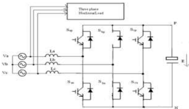
Fig.3 Power stage of a three-phase APF during 0\sim 60^\circ regions.
