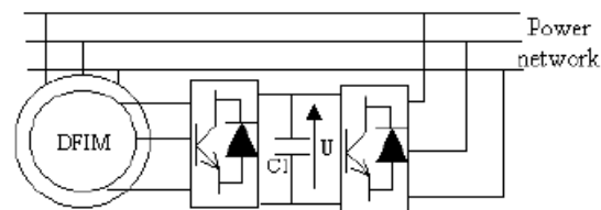
Fig. 1 Doubly-fed induction generator
