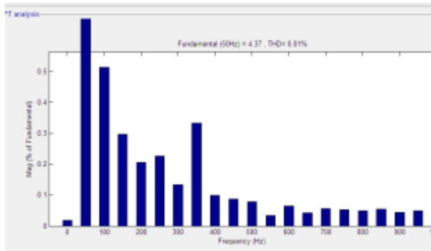
Fig.19. FFT analysis of fuzzy based shunt APF THD- 0.81%
