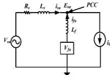
Fig.2. Single-phase equivalent circuit of APF topology.
