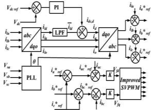
Fig.3. Proposed SVPWM control for APF topology.
