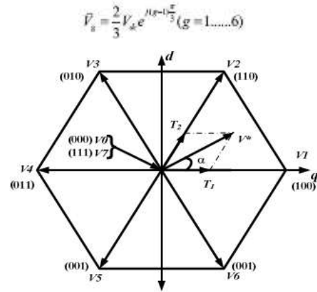
Fig.4.VSI Switching States Vectors.
