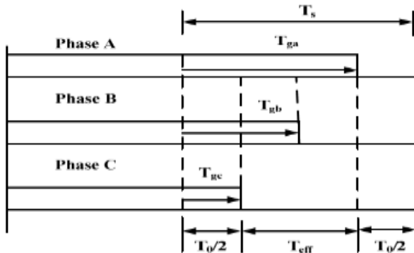
Fig.5. Proposed shunt APF switching pattern.
