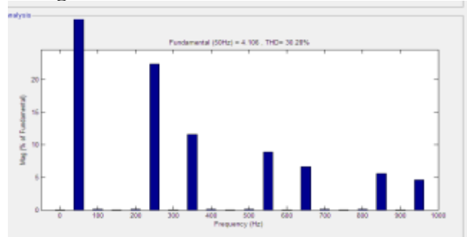
Fig.15. FFT analysis of without shunt APF THD-30.28%.
