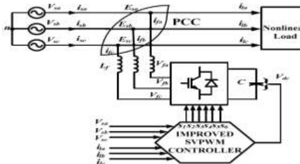
Fig.1. Configuration of Improved
