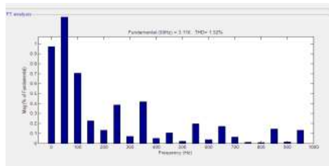
Fig.16. FFT analysis of with shunt APF THD-1.52%
