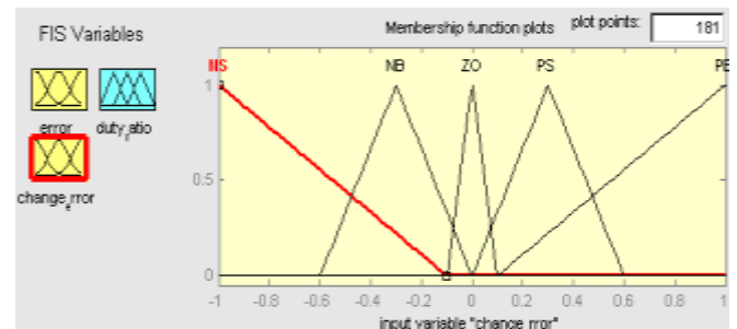
Fig.9. The Membership Function plots of change error.
