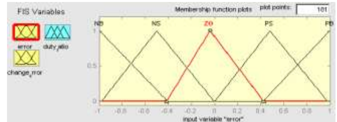
Fig.8. The Membership Function plots of error.
