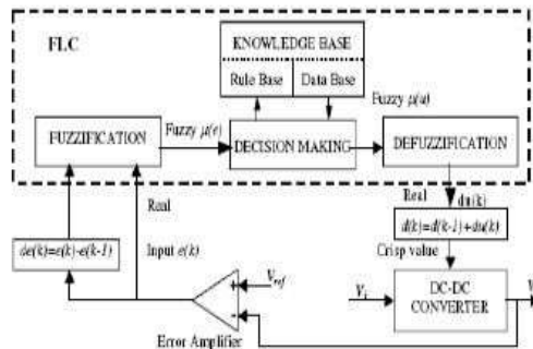
Fig.7. Block diagram of the Fuzzy Logic Controller (FLC) for dc-dc converters.
