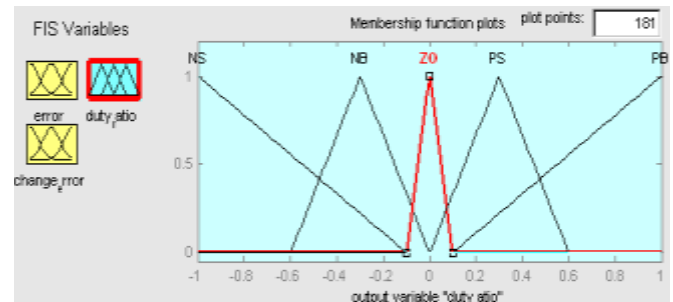
Fig.10. The Membership Function plots of duty ratio.
