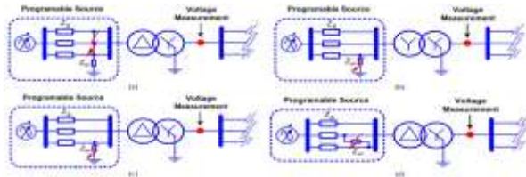
Fig. 1. Generation of grid voltage sags in the experimental setup. (a) Generation of a Type "A" voltage sag. (b) Generation of a Type "B" voltage sag. (c) Generation of a Type "C" voltage sag. (d) Generation of a Type "D" voltage sag
