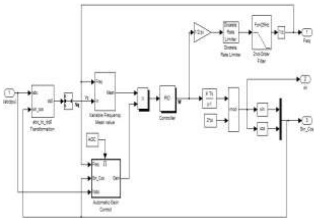
Fig Discrete phase PLL
