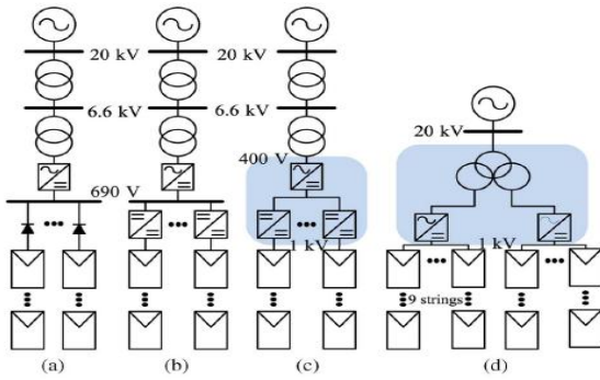
Fig. 1. Large-scale PV system configurations.
