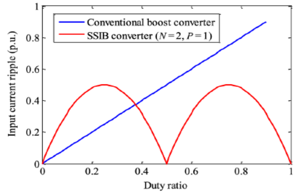
Fig. 5. Input current ripple of SSIB converter ( N = 2, P = 1 ) and conventional boost converter.
