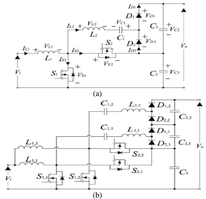
Figure 3. Converter topology. (a) SSB converter. (b) SSIB converter ( N = 2, P = 1 ).
