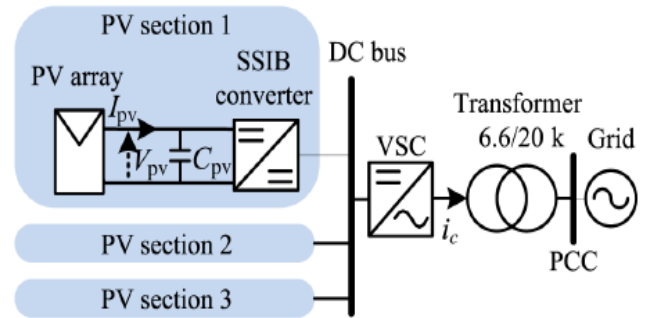
Fig. 2. Large-scale PV system architecture.
