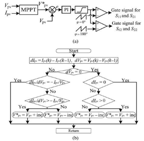
Fig. 6. Control block diagram. (a) N = 2 , P = 1 SSIB converter control loop. (b) Incremental conductance MPPT algorithm
