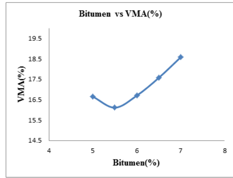
Fig-7: Variation of Bitumen Content for Stability & Air Voids
