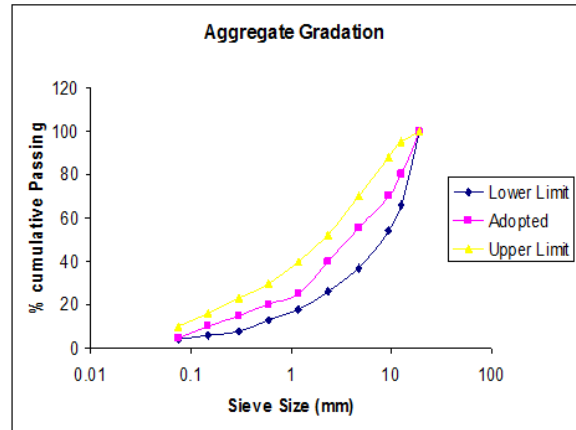
Fig-2: Aggregate Gradation for BC mix grade - II
