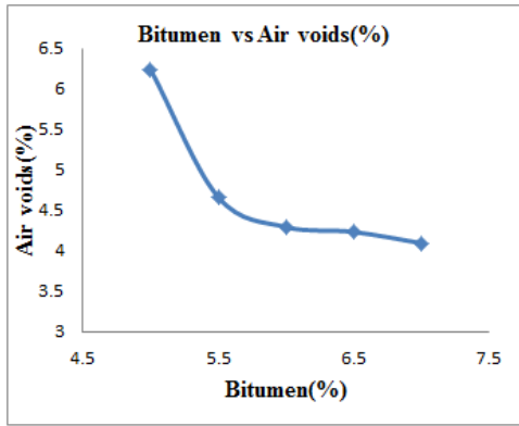
Fig-5: Variation of Bitumen Content for Stability and Air Voids
