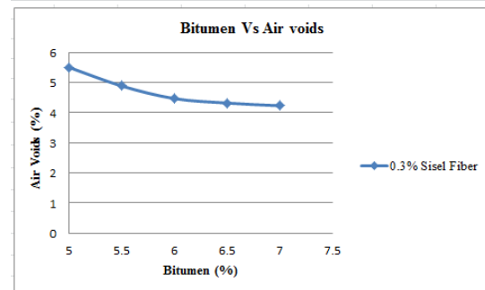
Fig-8: Variation of Bitumen Content for Stability & Air voids for RA mix.
