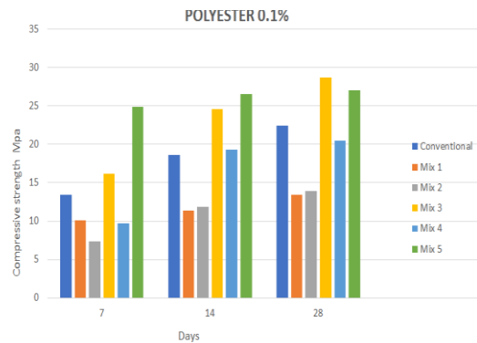
Figure 1 : Compressive strength
