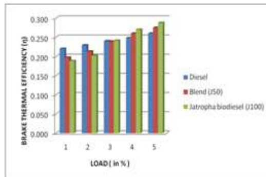
Fig 8 Variation of Brake Thermal Efficiency with Load
