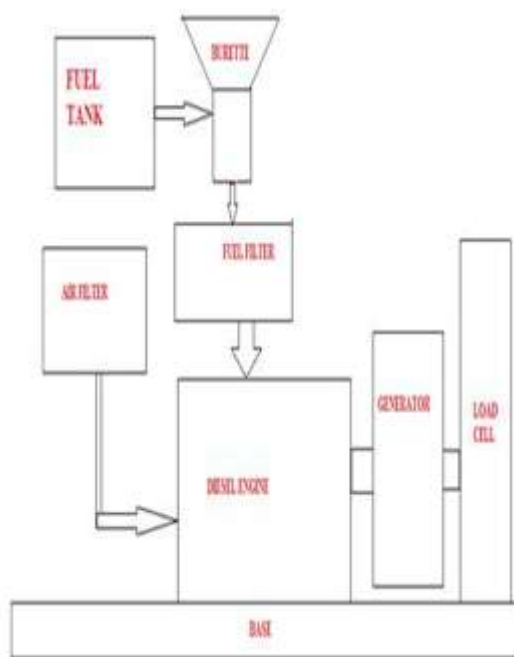
Fig. 5 A schematic diagram of the experimental set up
