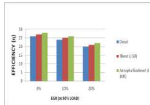
Fig 10 Effect of Exhaust Gas Recirculation on Efficiency at 80% load
