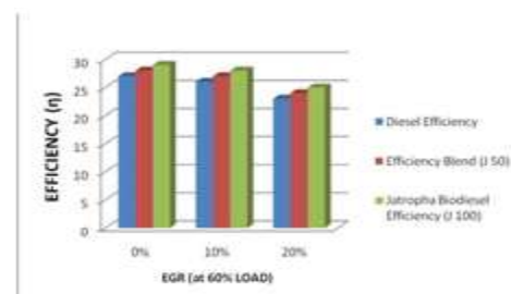
Fig 11 Effect of Exhaust Gas Recirculation on Efficiency at 60% load
