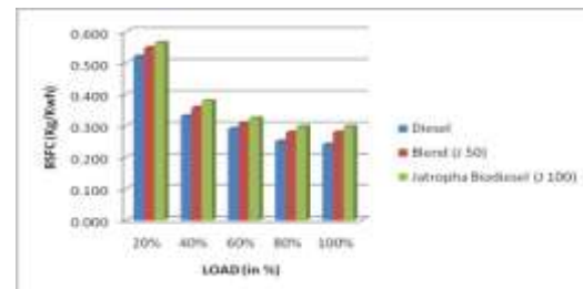
Fig 7 Variation of brake specific fuel consumption with load
