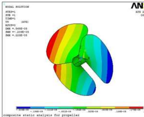
Deflection of a composite propeller with 8 layers direction
