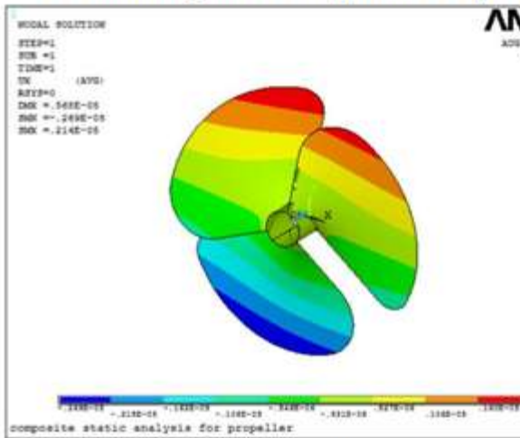
Deflection of a composite propeller with 8 layer direction
