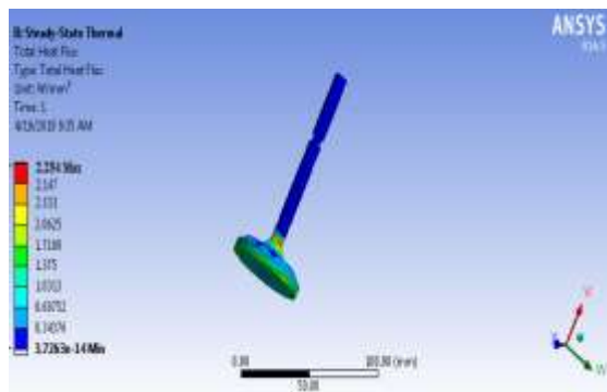
Figure.3 Total Heatflux For Nimonic 105
