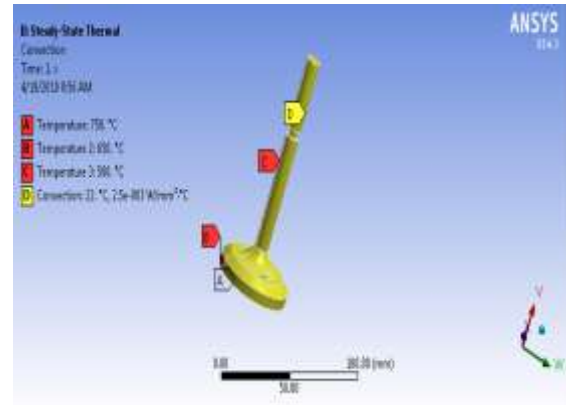
Figure.10 Boundary conditions and loads at thermal analysis
