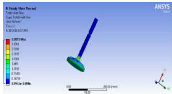
Figure.3 Total Heatflux For Nimonic 105
