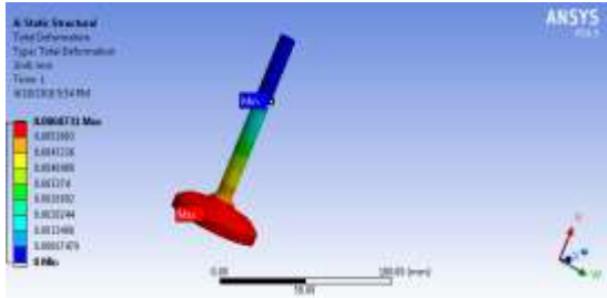
Figure.5 Total deformation for Nimonic 80a
