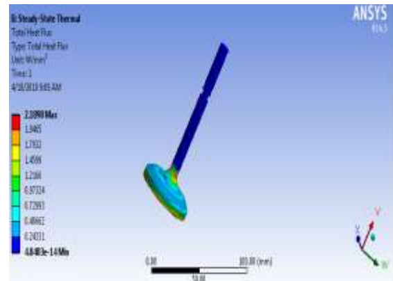
Figure.11 Total Heatflux For Stainless Steel
