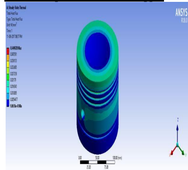
Figure 1 shows total heat flux piston with COPPER
