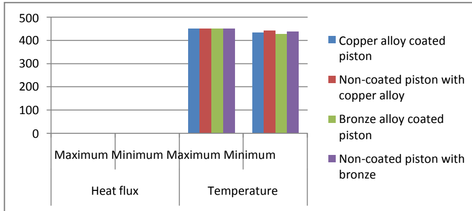
Graph 3 Comparison of Copper and Bronze Coated and Non Coated Piston Variations
