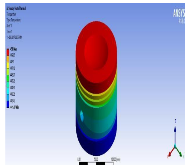
Figure 2 shows temperature variance piston with COPPER
