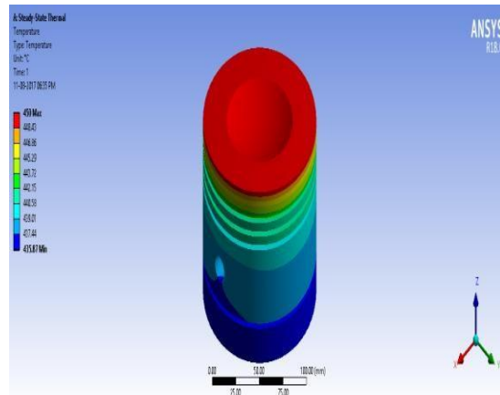
Figure 4 shows temperature variance piston with BRONZE
