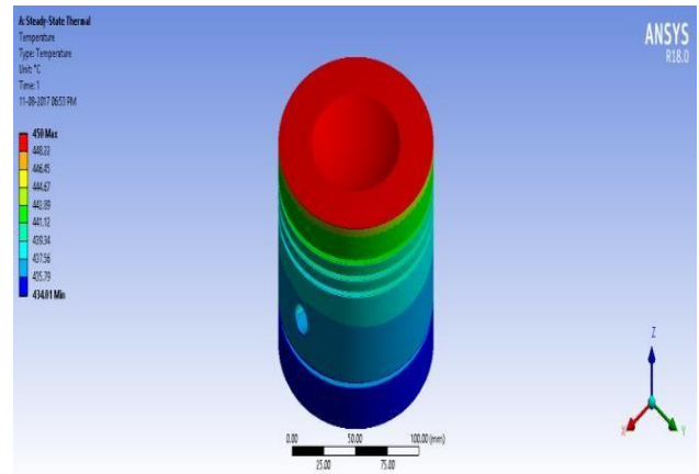
Figure 6 shows total temperature piston with crown of COPPER COATED PISTONMATERIAL AS BRONZE:
