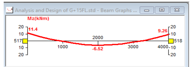
Figure shows the graph results of the high raised building at WIND LOAD along X-axis is applied
