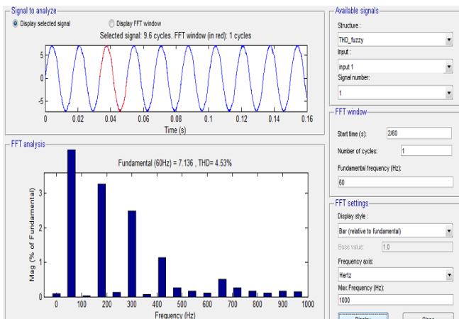
Fig 18 % THD using Fuzzy logic controller
