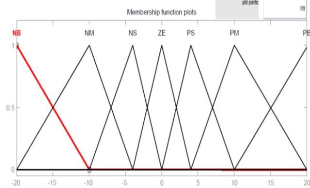
Fig.6 Membership Function of output
