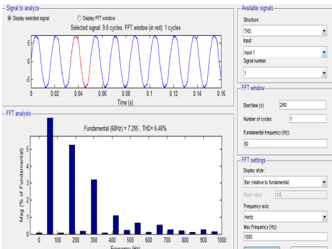
Fig 17 % THD using PI controller
