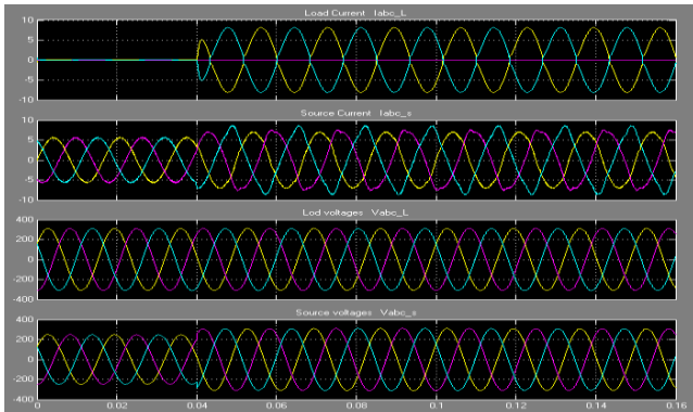
Fig. 16.iUPQC transitory response during the connection of a two-phase diode rectifier: (a) load currents, (b) source currents, (c) load voltages, and (d) source voltages
