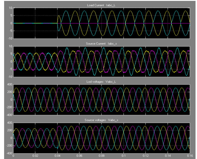
Fig. 14.iUPQC transitory response during the connection of a two phase diode rectifier: (a) load currents, (b) source currents, (c) load voltages, and (d) source voltages
