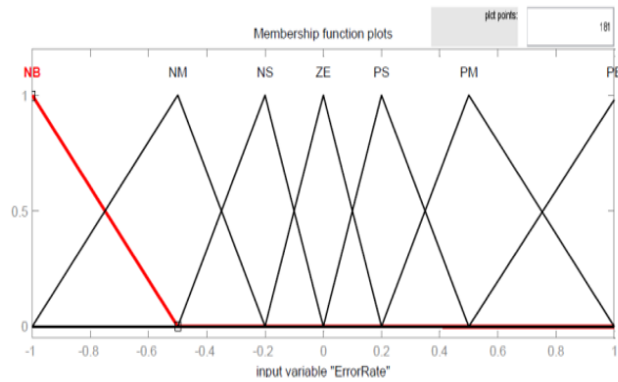
Fig.5 Membership Function of derivative error
