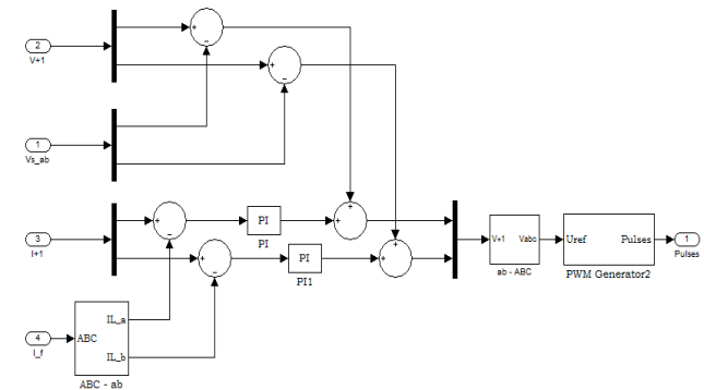
Fig10 simulation circuit of the voltage controller PWM iupqc
