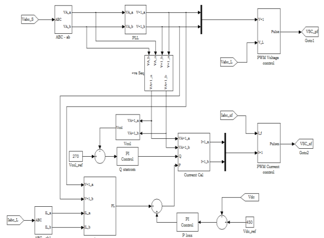
Fig 8 simulation circuit of the novel iUPQC controller
