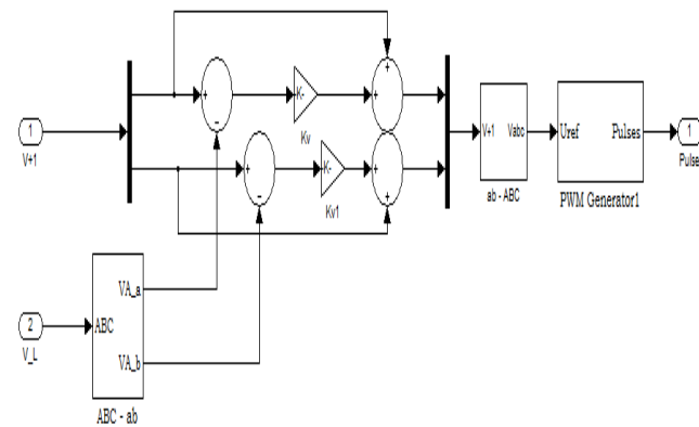
Fig10 simulation circuit of the voltage controller PWM iupqc
