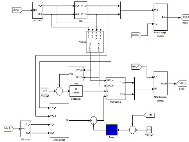
Fig 9 simulation circuit of the Fuzzy controller iupqc
