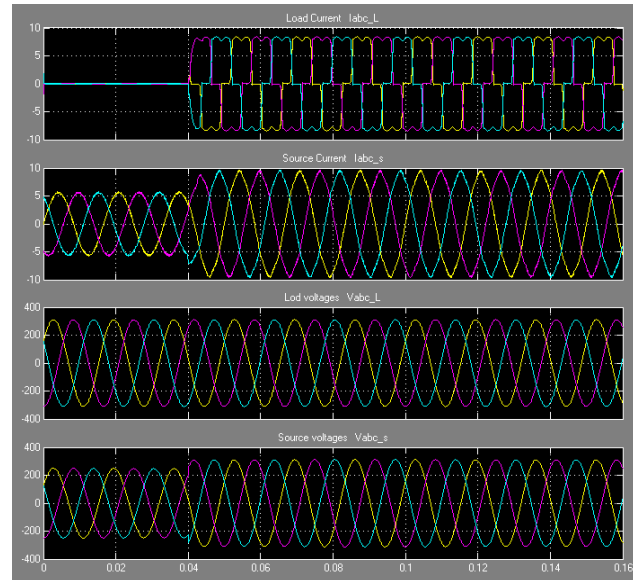
Fig. 13.iUPQC transitory response during the connection of a three phase diode rectifier: (a) load currents, (b) grid currents, (c) load voltages and (d) grid voltages.
