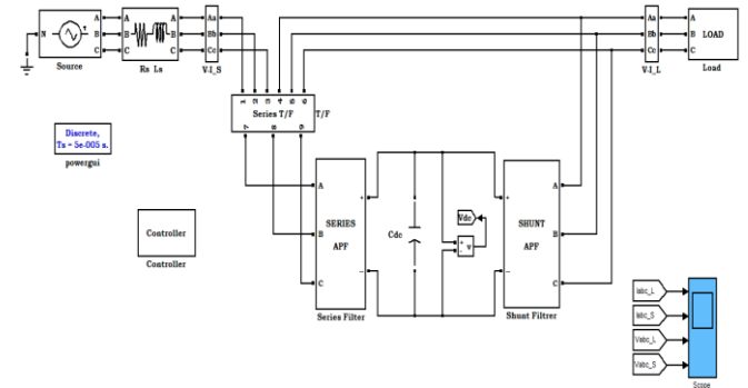
Fig 7simulation circuit of proposed system
