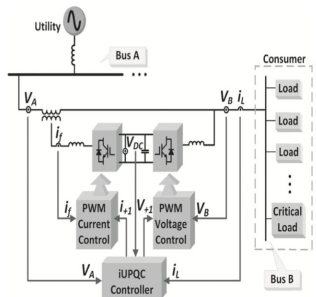
Fig. 2 Proposed iUPQC configuration.
