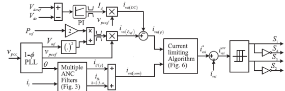
Fig.6 Block diagram of the proposed multiple ANC-filters-based control scheme.
