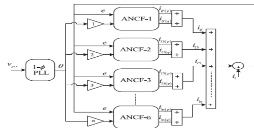
Fig.5 Block diagram of multiple ANC filters-based fundamental extraction.
