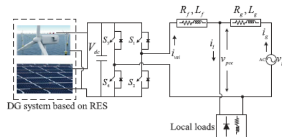
Fig.3 Schematic of single-phase GCI system.
