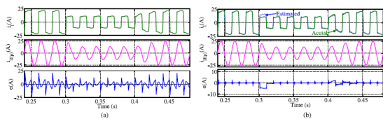
Fig.5.1 Extraction of fundamental active power component of load current using (a) Single ANC filter. (b) Multiple ANC filters.
