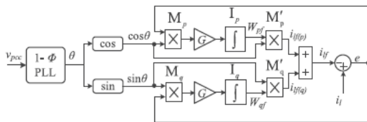
Fig.4 ANC filter.
