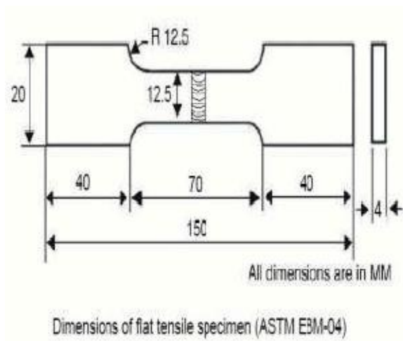
Fig 13: Tensile test specimen
