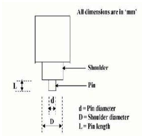
Fig11: Tool details
