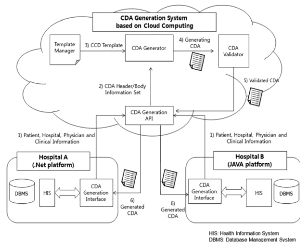
Fig. 1. The architecture of our CDA generation system based on cloud computing.
