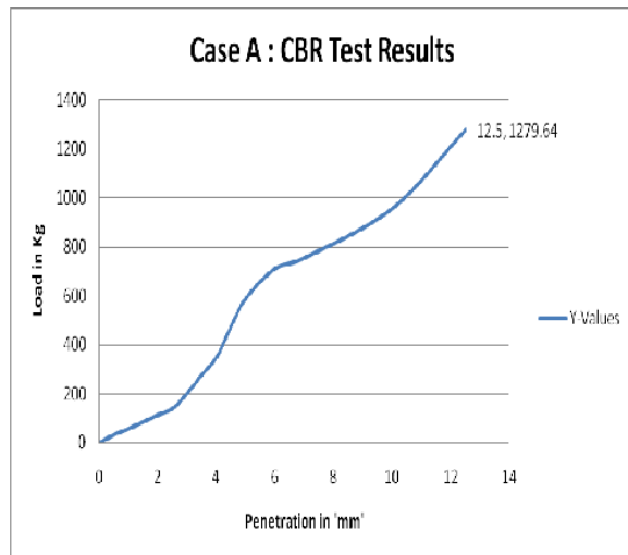
Figure 4.9 CBR test results for Case A CBR for 2.5mm penetration =12.4% CBR for 5mm penetration=10.7%
