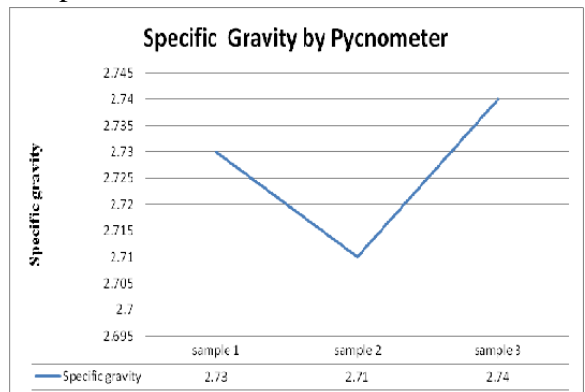
Figure 4.1(b) Specific gravity of soil samples
