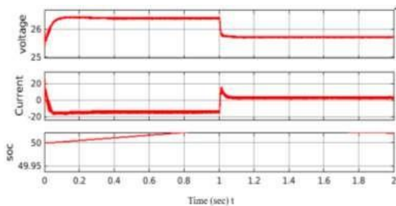
Figure 7. Output of Battery
