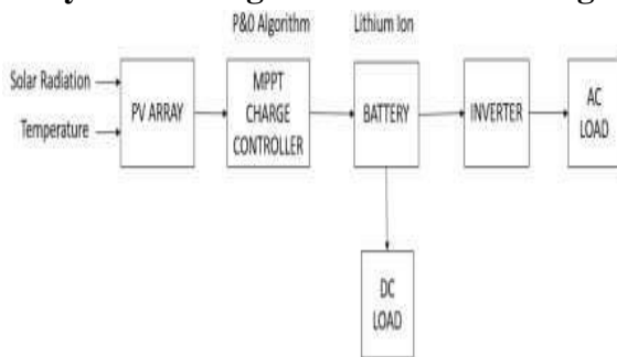
Figure 1. Block Diagram of Battery Management for Solar PV standalone System
