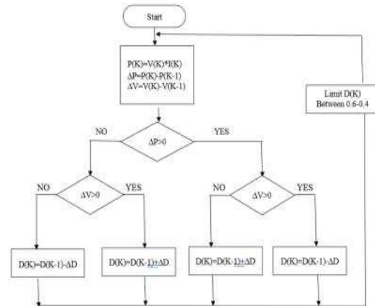
Figure 3.P & O MPPT Scheme
