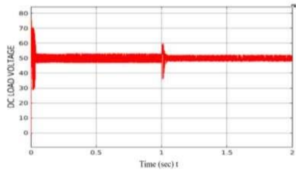
Figure 8. DC Voltage across Load
