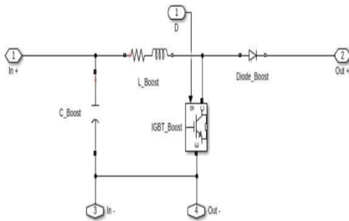
Figure 4. Circuit Diagram of DC-to-DC Converter (BOOST) used in simulation
