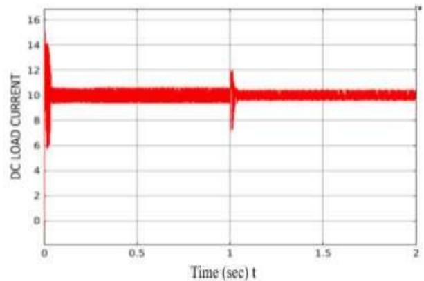
Figure 9. DC Current across Load
