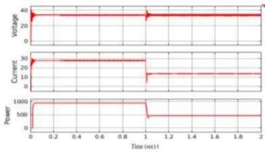
Figure 6. Output result of solar PV
