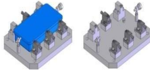
Figure 1 Typical fixture with workpiece
