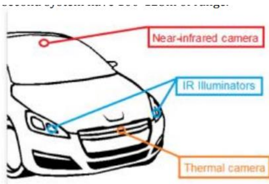
Fig 4: Camera placement of high-quality night vision system
