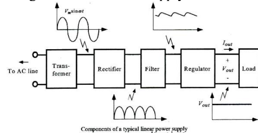
Fig: Block Diagram of Power Supply
