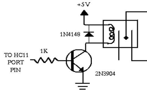
BASIC RELAY SWITCH
