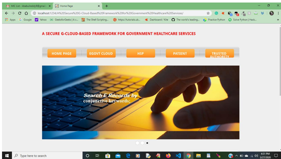
Fig 4.1 Home Page
