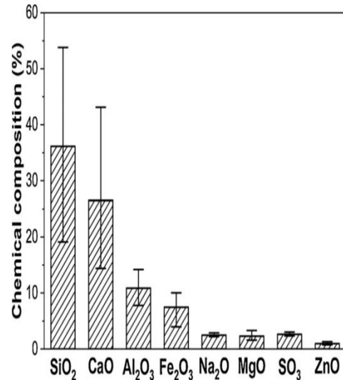
Fig. 2: (a). Chemical composition and mineralogy of MIBA: Chemical composition
