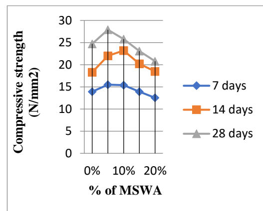
Fig. 8: Compressive strength v/s % of MSWA.
