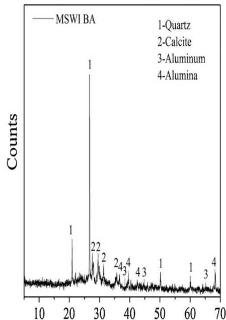
Fig. 3: (b). Chemical composition and mineralogy of MIBA: XRD
