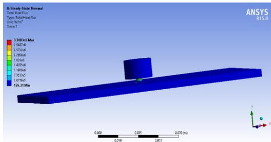
Total heat flux for tapered tool
