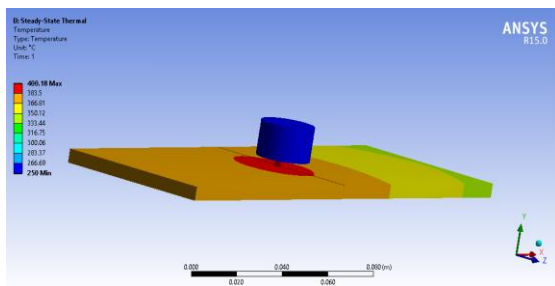
Total temperature for circular tool
