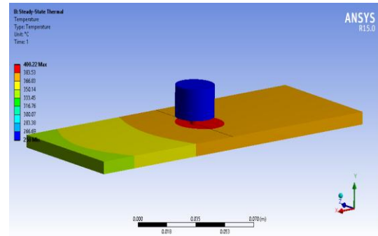
Total temperature for truncated tool
