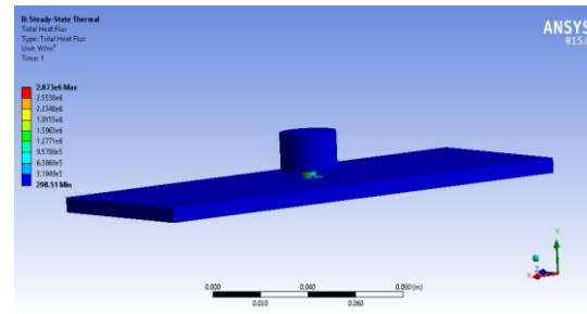
Total heat flux for truncated tool
