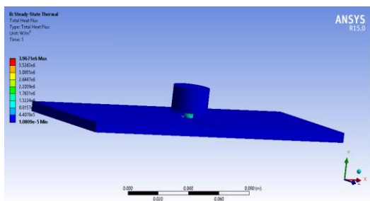
Total Heat Flux Values for Circular Tool
