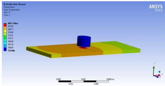
Total temperature for tapered tool
