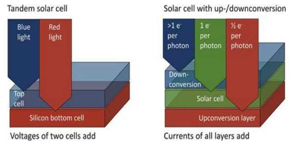
FIG. 1. Working principle of a tandem solar cell (left) and an up- and downconversion-based solar cell (right). The tandem cell consists of two separate sub-cells, often the bottom cell is made of silicon and absorbs the low-energy part of the solar spectrum, and the top cell absorbs the higher-energy photons. The up- and down conversion cell often only consists of one solar cell junction, while the up- and downconversion layers transform the incident spectrum so that it can be better converted by the cell.
