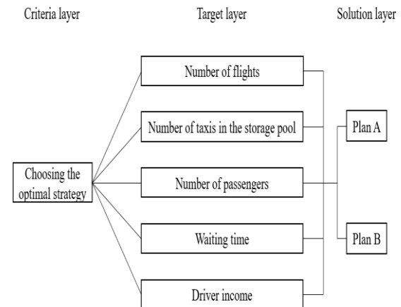
Figure 1. Hierarchy chart
