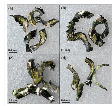
Figure 7. Chip morphology under different CL conditions:
