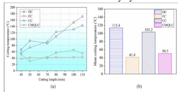
Figure 4. Cutting temperature variation with CL condition (a) and its average value (b).
