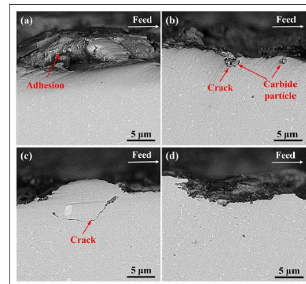
Figure 9. The metallographic structure under different CL conditions: (a) DC, (b) FC, (c) CC, and (d) CMQLC.
