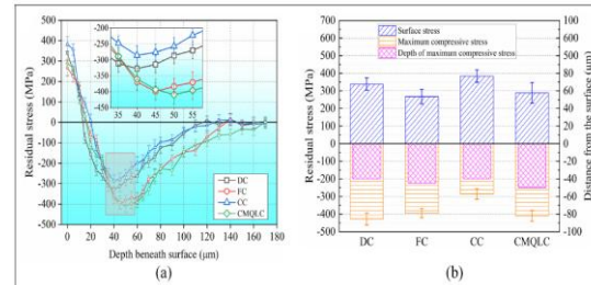
Figure 10. Residual stress under different CL conditions: (a) variation trend and (b) stress characterization.
