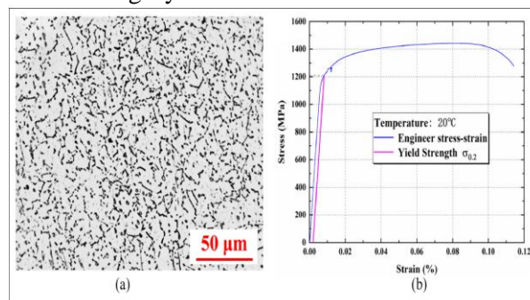
Figure 1. Microstructure and tensile properties of the Inconel 718 superalloy: (a) OM microstructure and (b) tensile stress-strain curve.
