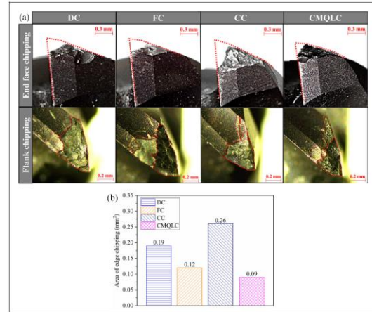
Figure 5. Tool chipping under different CL conditions: (a) topography of edge chipping and (b) areas of flank chipping.
