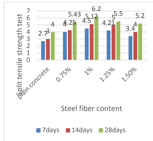
Graph 5.4. Split tensile strength test for varying steel content
