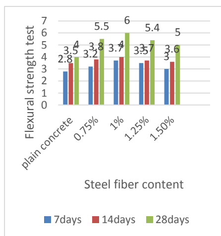
Graph 5.5. flexural strength test result for varying steel fiber content
