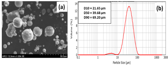
Figure 2. (a) SEM images, and (b) Particle size distribution of AlSi10Mg powder
