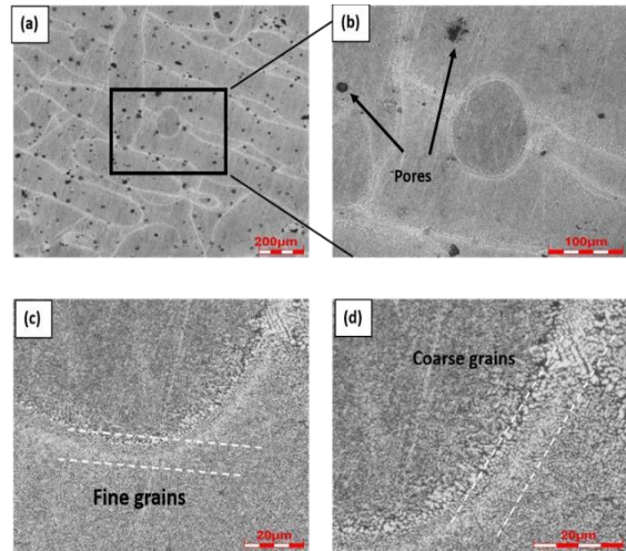
Figure 4. Optical images of AlSi10Mg @ 60 µm layer thickness (a) microstructure @ 200X (b) Microstructure @ 693X magnification and (c)Microstructure @ 2000X magnification (d) microstructure @4000X
