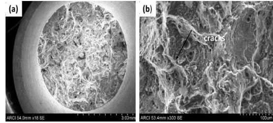
Fig 9. SEM fractography micrographs of 60 \mu m vertical built
