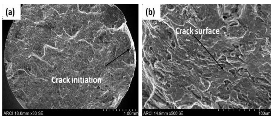
Fig 8. SEM fractography micrographs of 30 \mu m horizontal built
