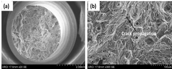
Fig 7. SEM fractography micrographs of 60 \mu m horizontal built
