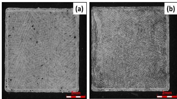
Figure 3. Top view of micro structure of AM built AlSi10Mg (a) 60 µm (b) 30µm
